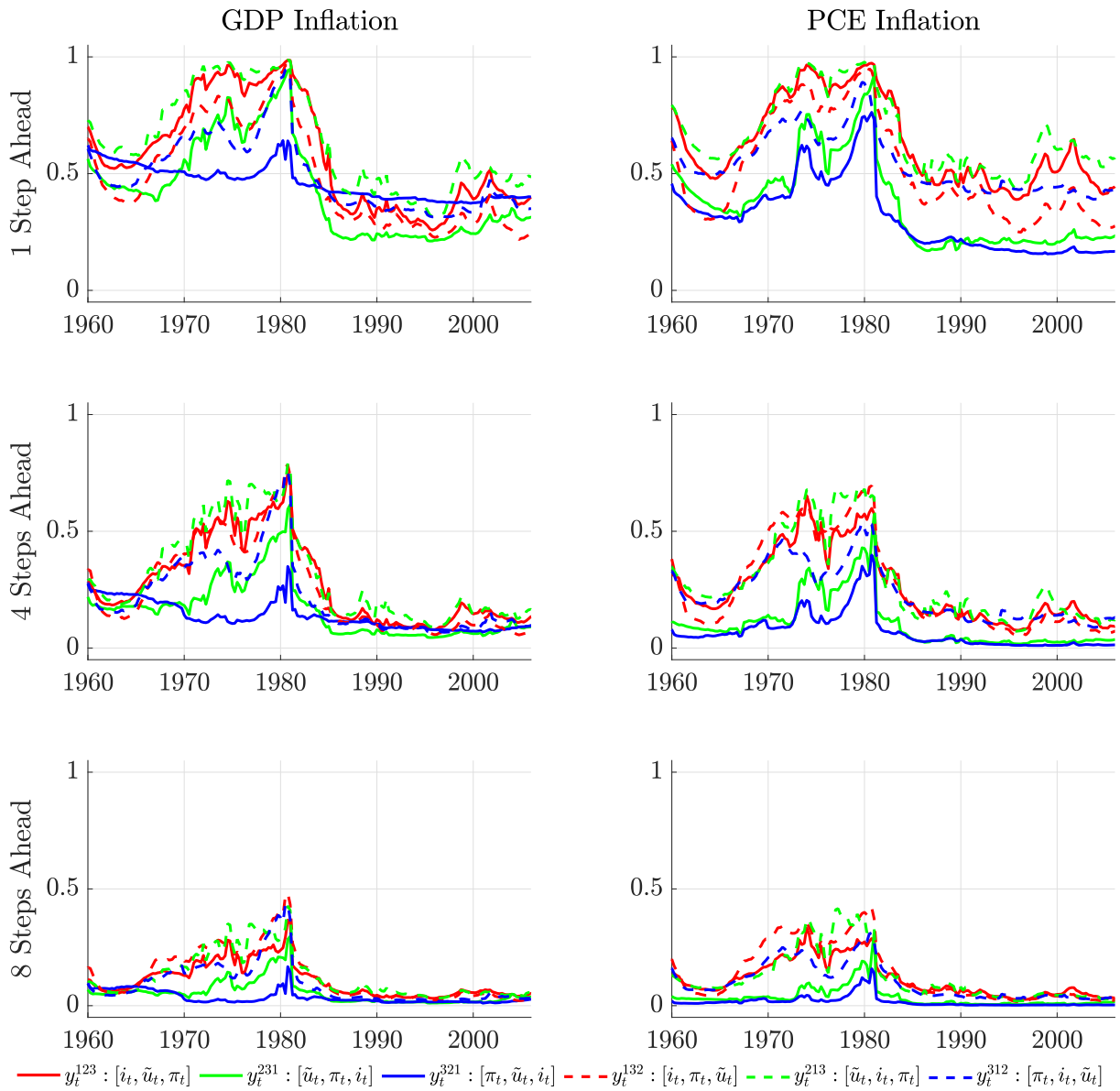
Figure 4: R_{j,t}^2 statistics
