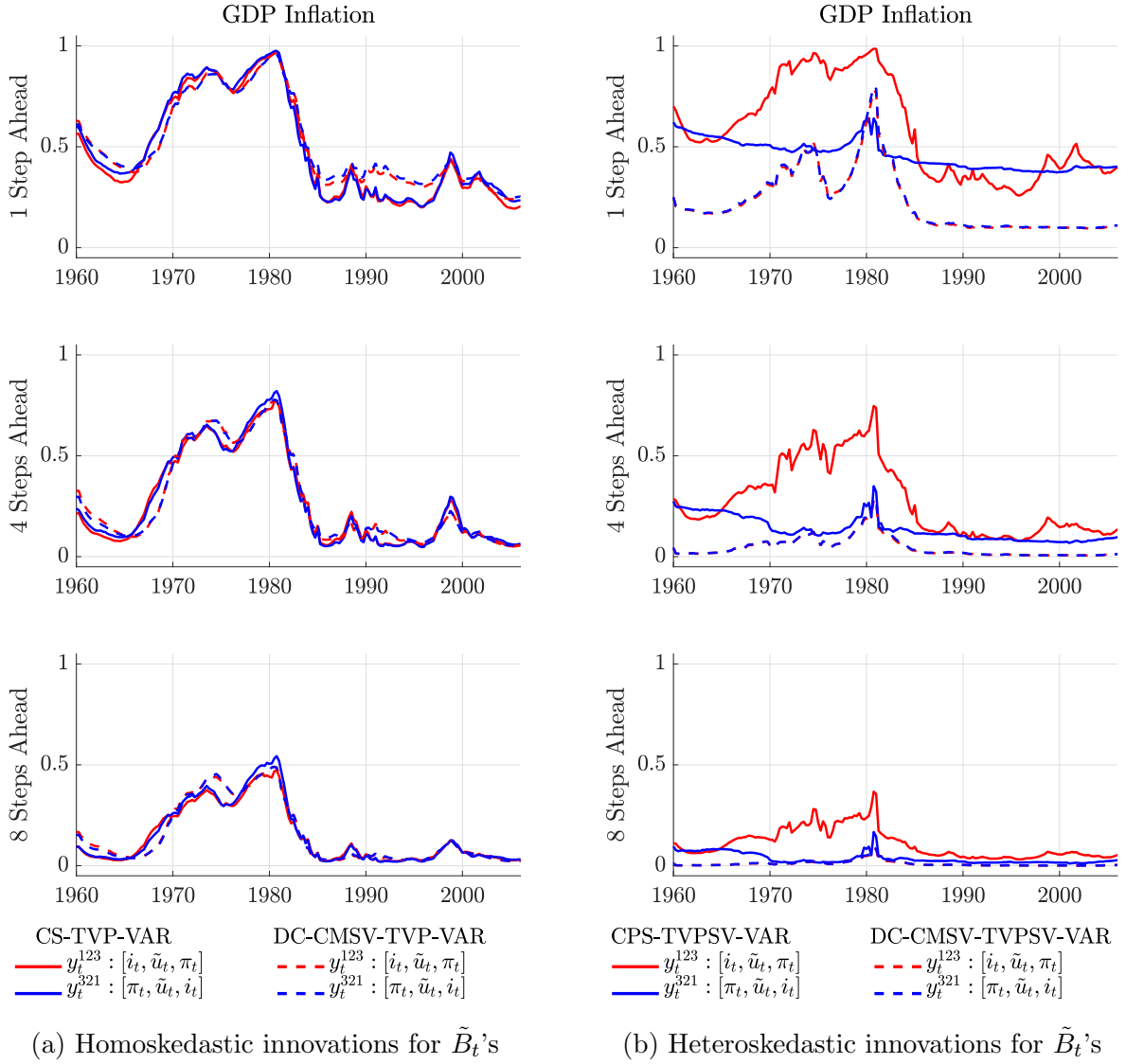
Figure 5: R_{j,t}^2 statistics
