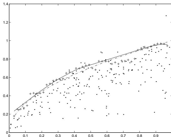
Figure 2: Stochastic DEA: one sample of size n = 200 . The true frontier is the dash dot line. The \cdot 's represent the observations, the + 's are the point wise estimates of the boundary over a selected grid of 48 values for x , the solid line is the stochastic DEA. Here \rho_{nts} = \sigma_W/\sigma_V = 0.40 .
