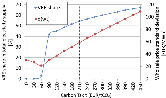
(b) VRE supply share in total annual electricity and standard deviation of the wholesale price \sigma(w_t) for increasing carbon taxes \tau
