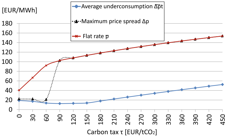
Fig. 4 Average under-consumption \overline{\Delta p_t} , maximum retail price spread \Delta p , and flat retail rate across carbon tax scenarios
