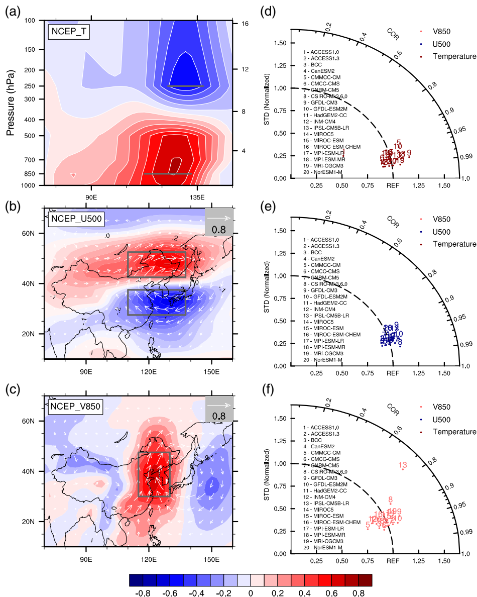
FIGURE 1 Performance of CMIP5 models in simulating meteorological anomalies ( HWI > 0 ) during 1986–2005 period. Based on NCEP datasets: (a) 40^\circ\text{N} vertical section distribution anomaly of atmospheric temperature with HWI > 0 ; (b) 500 hPa wind anomaly with HWI > 0 , shading indicates zonal flow; (c) 850 hPa wind anomaly with HWI > 0 , shading indicates meridional flow; (d)–(f) the correlation coefficients (the arc) and standard deviation (the x-axis) between each of the CMIP5 models and the NCEP datasets of the three meteorological anomalies using Taylor diagrams
