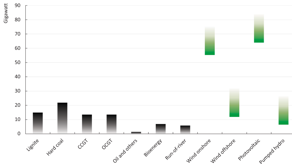
Fig. 1. Assumptions on upper and lower bounds for the generation portfolio. Dispatchable thermal and run-of-river generation capacity (black) can be installed up to the specified upper bound; in contrast, variable renewable and pumped hydro storage capacity (green) face a lower installation bound
