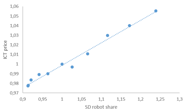
Figure 4: Standard deviation of robot share across applications versus ICT price index, 2005-2015 (2005=1).
