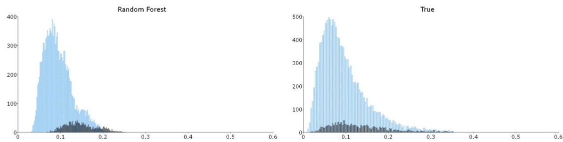
Figure 2: Propensity scores by treatment status, N=16,000, 10% treated
