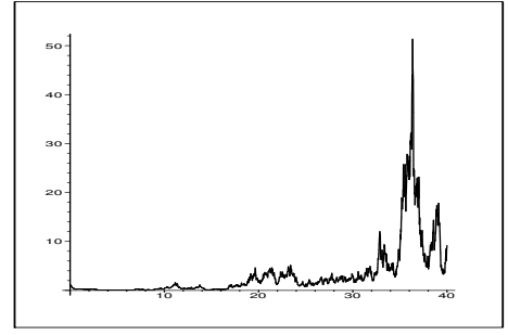
Figure 1: dX(t) = \{0.35X(t) + 0.1X(t - 1)\}dt + \sigma X(t)dW(t) , \psi \equiv 1 , \sigma = 0 (left) and \sigma = 0.8 (right).
