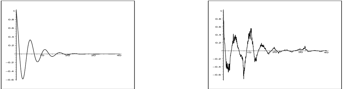
Figure 3: dX(t) = \{0.35X(t) - X(t - 1)\}dt + \sigma X(t)dW(t) , \psi \equiv 1 , \sigma = 0 (left) and \sigma = 0.8 (right).
