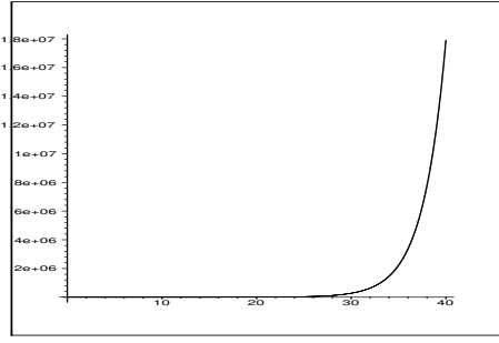
Figure 1: dX(t) = \{0.35X(t) + 0.1X(t - 1)\}dt + \sigma X(t)dW(t) , \psi \equiv 1 , \sigma = 0 (left) and \sigma = 0.8 (right).
