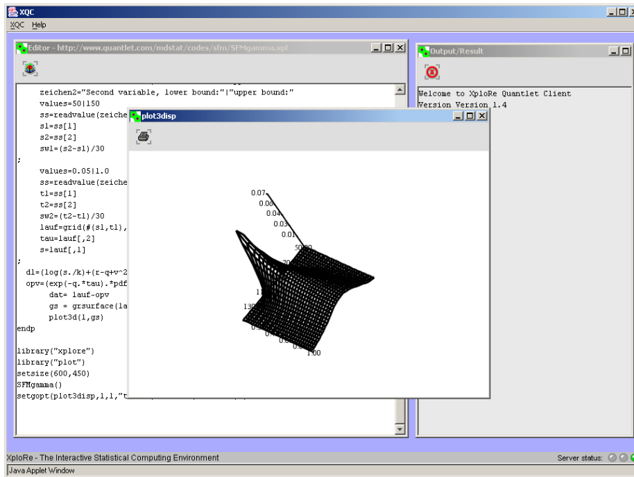
Figure 4: The output of SFgamma.xpl in the XQC edit-version
