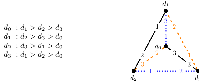
Fig. 1. An instance that admits two popular matchings—marked by dotted blue and dashed orange edges—but no stable matching. The preference list of each vertex is illustrated by the numbers on its edges: a lower number indicates a more preferred neighbor.
