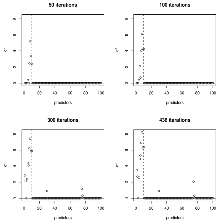
Fig. 5. Degrees of freedom ( df ) in additive model fitting for all 100 predictor variables (from model (14)) during the process of penalized L_2 Boosting with individual smoothing splines (having df = \text{trace}(\mathcal{S}_j) = 2.5 for each spline). The first ten predictor variables (separated by the dashed line) are effective. The result is based on one realization from model (14) with sample size n = 200 . The plot on the lower right corresponds to the estimated optimal number of boosting iterations using the AIC_c criterion in (12). Only three non-effective predictors have been selected (and assigned small amount of df ), and one effective predictor has not been selected (but whose true underlying function is close to the zero-line, see Figure 6).
