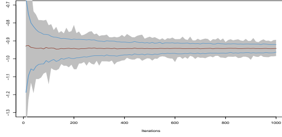
Fig. 2. Evolution of a sequence of 500 estimators (6) over 1,000 iterations: range ( in gray ), .05 and .95 quantiles, and average, obtained on the same sample as in Figure 1 when simulating from the t distribution with location x_1 .
