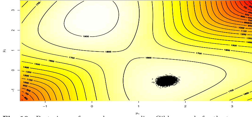
Fig. 10. Posterior surface and corresponding Gibbs sample for the two mean mixture model, when initialized close to the second and lower mode, based on 10,000 iterations ( Source: Robert and Casella, 2004 ).
