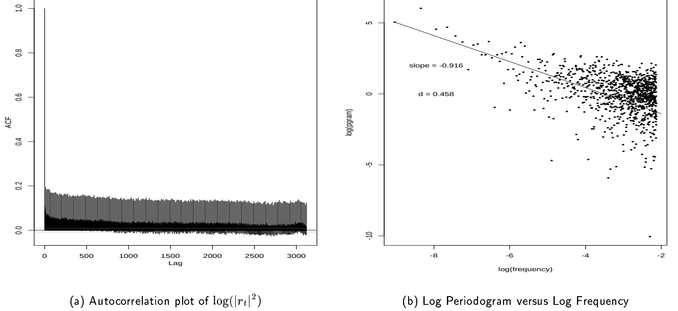
Figure 5: Autocorrelations and log(Periodogram) of \log(|r_t|^2)
