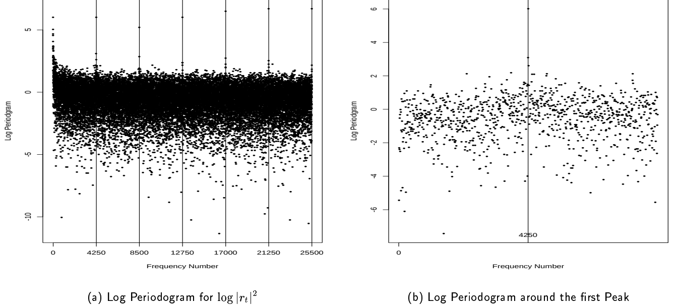
Figure 2: Log Periodogram for High Frequency Log Squared Returns
