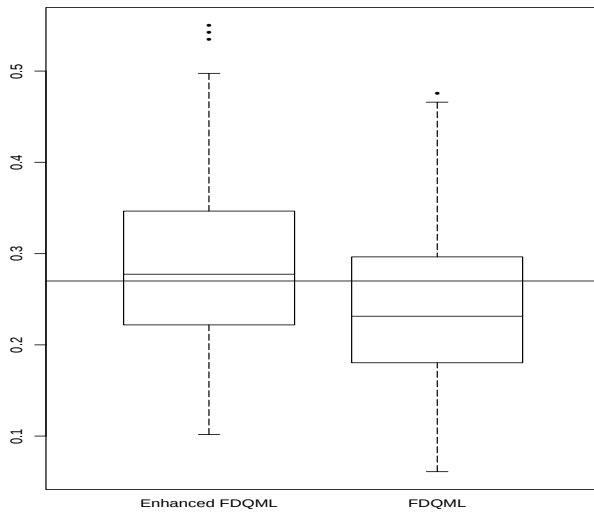
(c) \hat{\sigma}_\eta^2 ( \sigma_\eta^2 = 0.27 )
