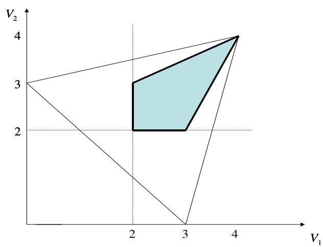
Figure 3: Stag Hunt
