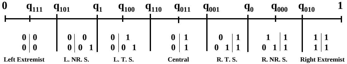
Figure 3: Path of play of class 0 and class 1 equilibria in the two-sender game.
