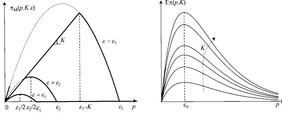
Figure 1: The sample path of \pi_M(p, K, \epsilon) as a function of p for three representative values of \epsilon : low ( \epsilon_1 ), medium ( \epsilon_2 ) and high ( \epsilon_3 ). On the right, we have E\pi_M(p, K, \epsilon) when \epsilon is exponentially distributed.
