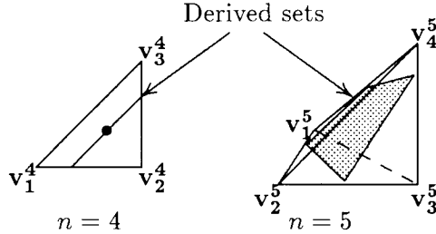
Fig. 1. Voting Pyramids \mathcal{P}^n
