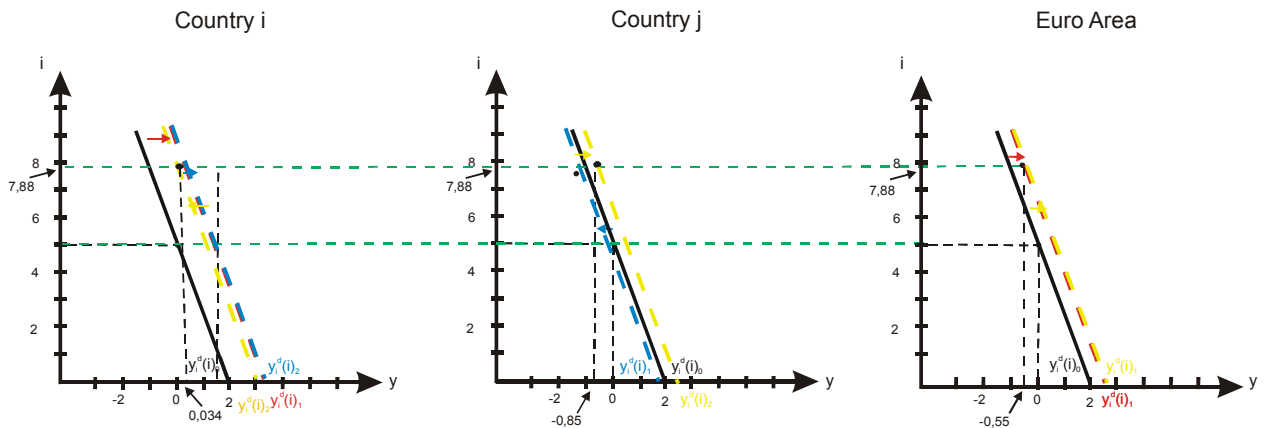
Figure 8: Idiosyncratic Supply Shocks in Country i : \varepsilon_{i,1} = 3
