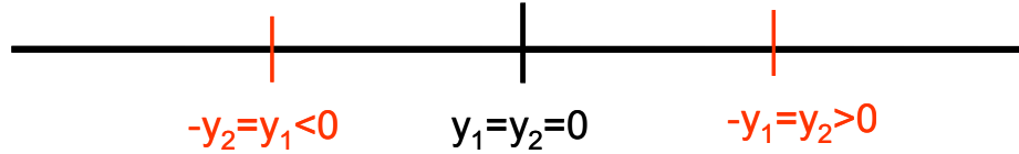
Figure 1: Mean Preserving Distribution of Macroeconomic Outcomes
