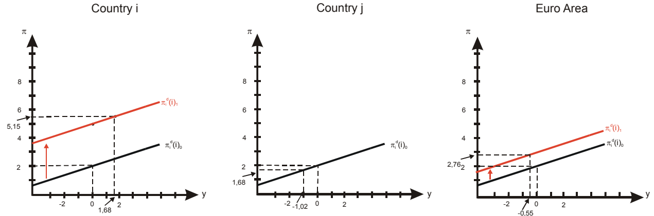
Figure 4: Idiosyncratic Supply Shock in Country i: \varepsilon_{2,i} = 3
