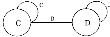
Figure 4.2.2 The skeleton of the automata in A .
