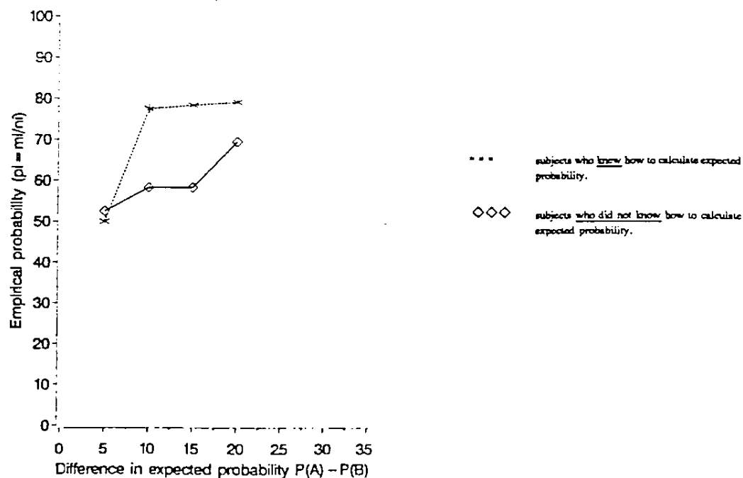
C - Risk neutral induced preferences
