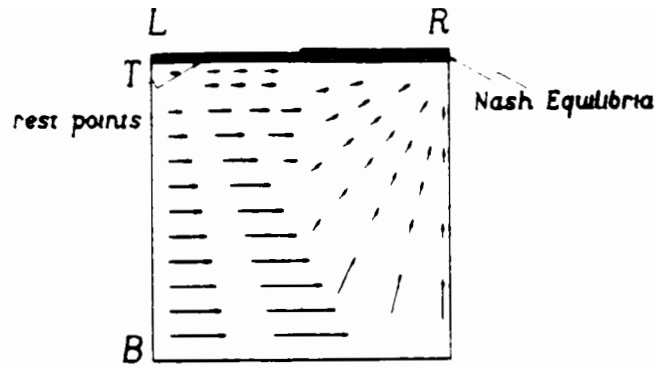
FIGURE 2: A myopic adjustment dynamic for G_1 under which T \times \Phi_2 is asymptotically stable.
