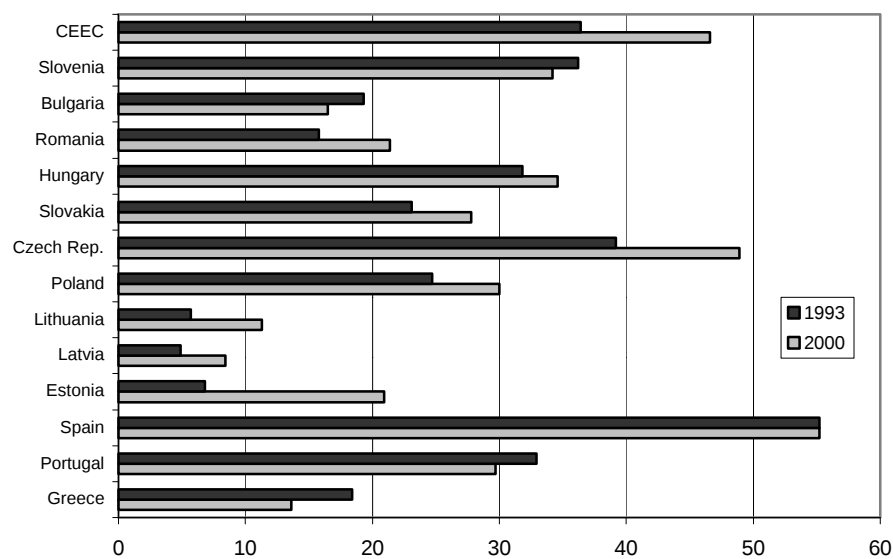
Figure 10: Intra-Industry Trade
