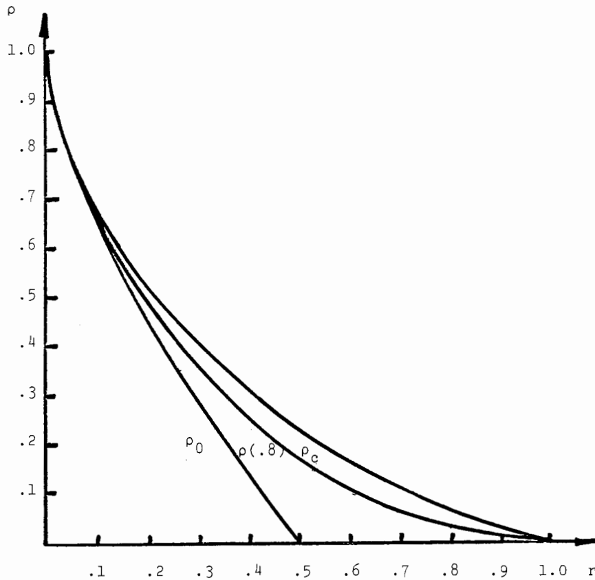
Figure 1: The Critical Numbers \rho_0 , \rho(.8) and \rho_c as functions of r
