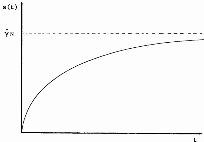
Figure 6 Sales For a Moderate Repeat Purchase Rate \gamma_1 > \bar{\gamma} > \mu or \gamma_1 < \bar{\gamma} < \mu
