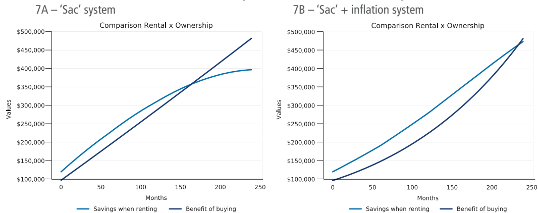
FIGURE 7 Plots of default simulation for 'sac' system and 'sac' + inflation system
