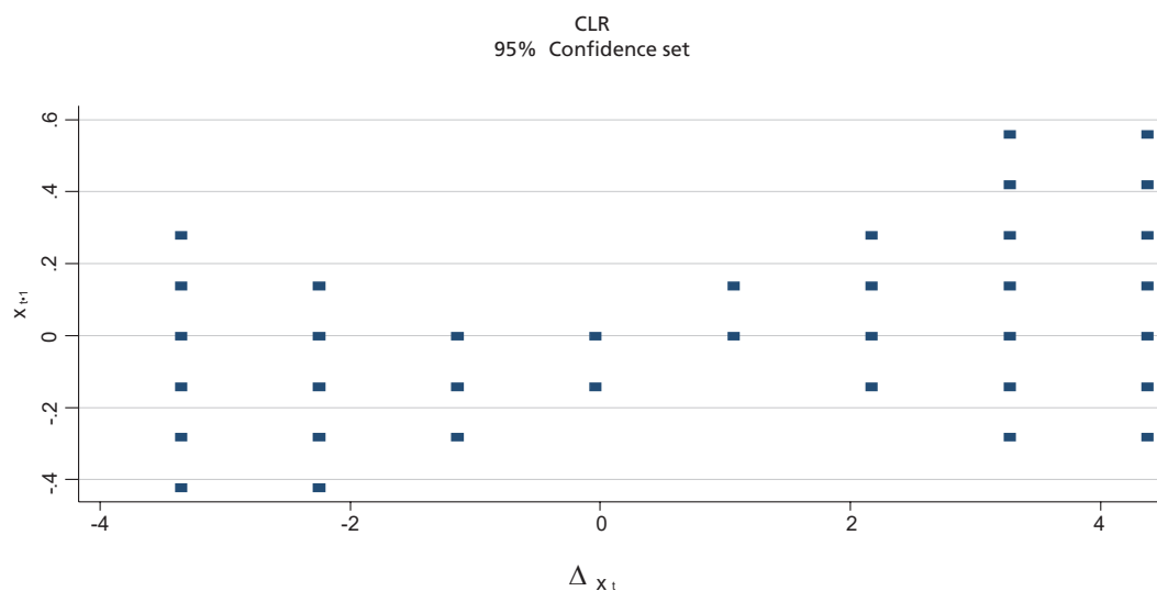
GRAPH 5 CLR robust confidence region for \Delta x_t and x_{t-1} .
