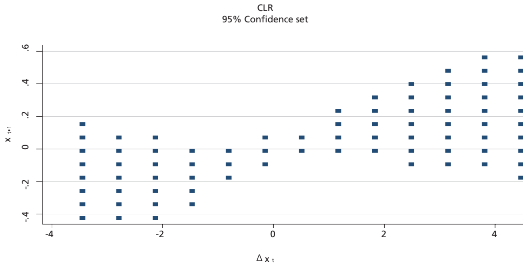
GRAPH 7 CLR robust confidence region for \Delta x_t and x_{t-1} for the restricted model where \delta_1 = 0 .
