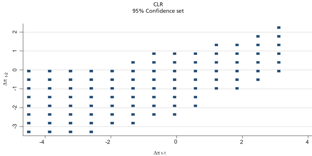
GRAPH 6 CLR robust confidence region for \Delta\pi_{t-1} and \Delta\pi_{t-2} for the restricted model where \delta_1 = 0 .
