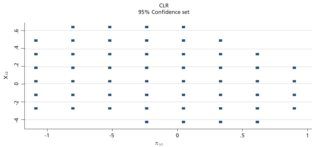
GRAPH 4 CLR robust confidence region for \pi_{t-1} and x_{t-1} .
