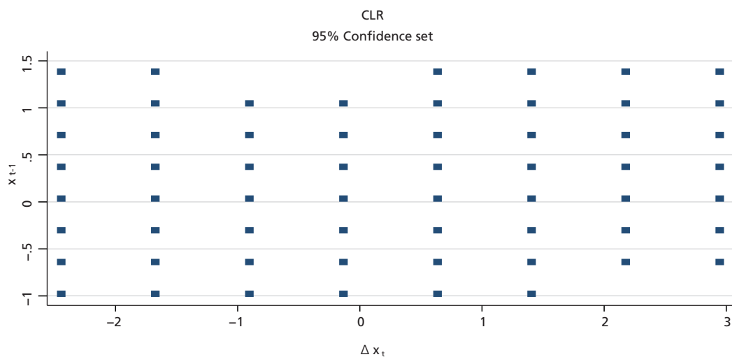
GRAPH 6 CLR robust confidence region for \Delta x_t and x_{t-1} .
