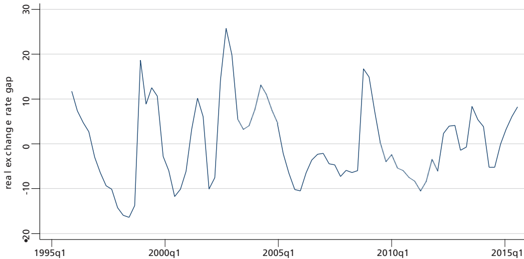
GRAPH 3 Real exchange rate gap
