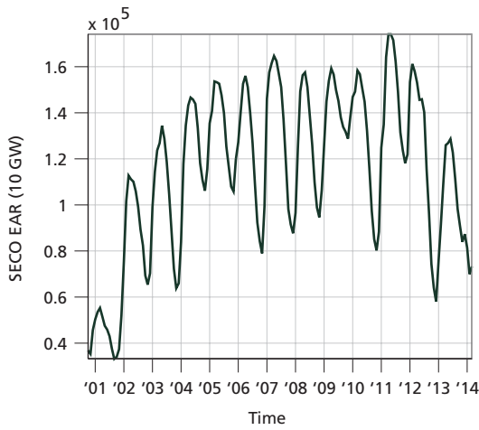
(a) Stored energy
