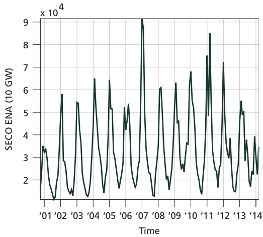
(a) Natural hydro power
