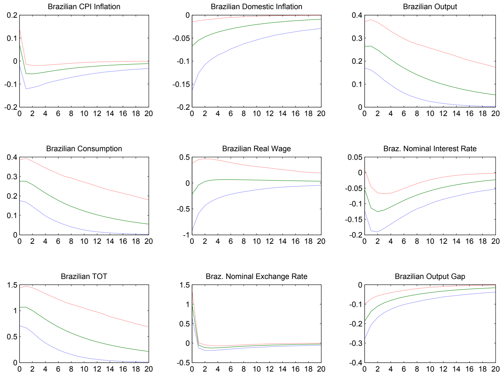
Figure 4: Impulse Response Functions to Brazilian Productivity Shock
