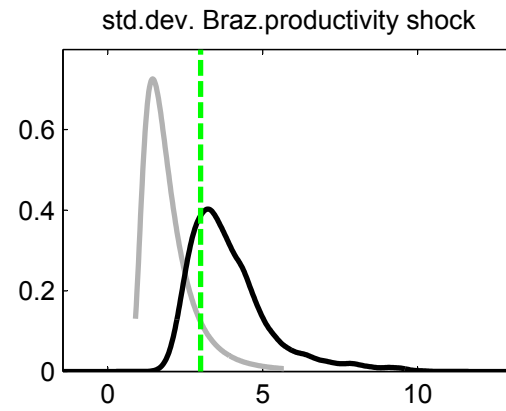
Figure 1: Prior and Posterior Densities
