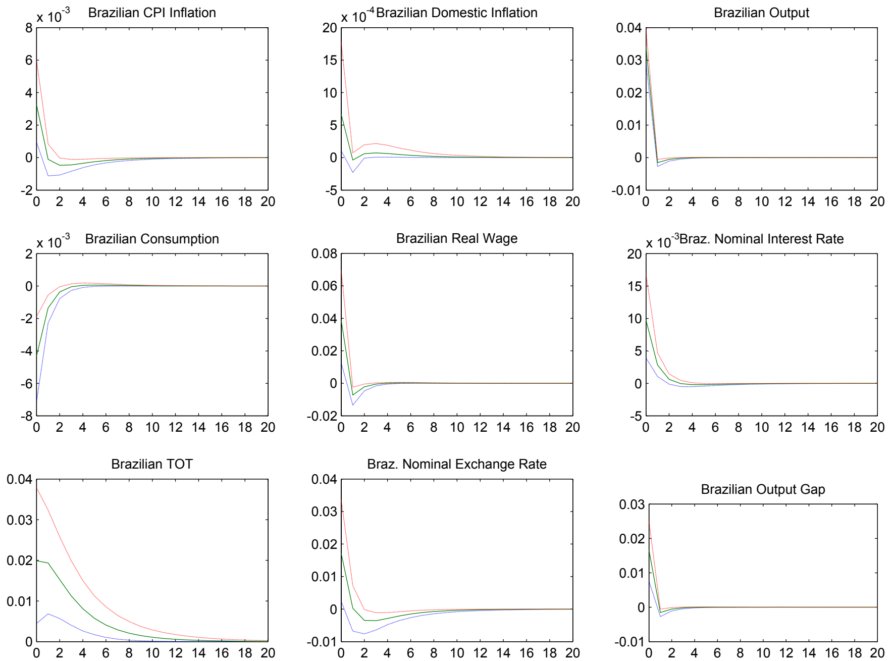
Figure 9: Impulse Response Functions to Risk Premium Shock
