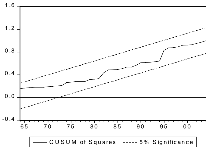
GRAPH 4 CUSUM OF SQUARES TEST: SAVING
