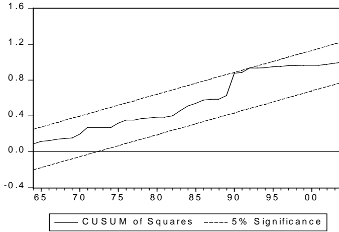
GRAPH 3 CUSUM OF SQUARES TEST: INVESTMENT
