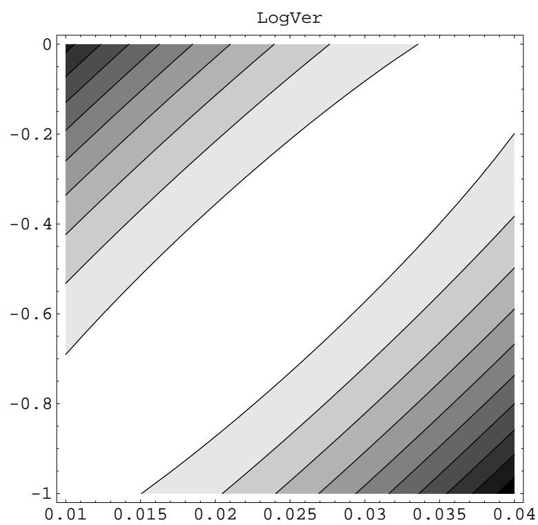
Figure 9: Graph of the log-likelihood when varying \theta^r \times \lambda^r around the maximum.
