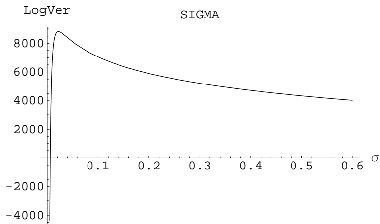
Figure 7: Variation of the log-likelihood changing \Sigma^{rr} around the maximum.
