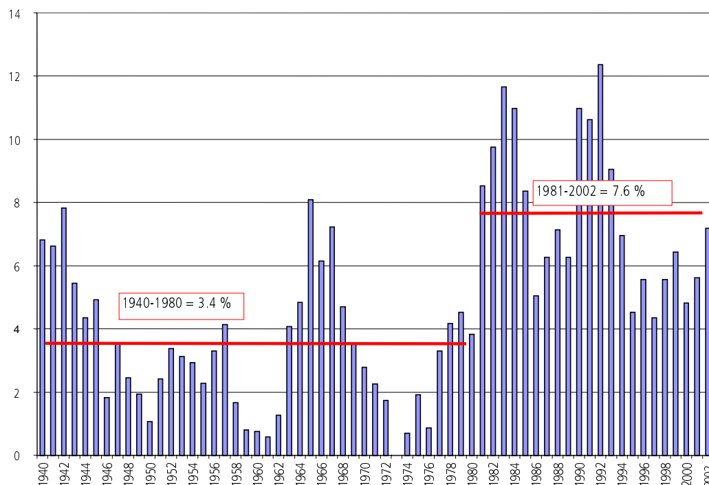
FIGURE 11 IDLE CAPACITY—1940-2002 [%]
