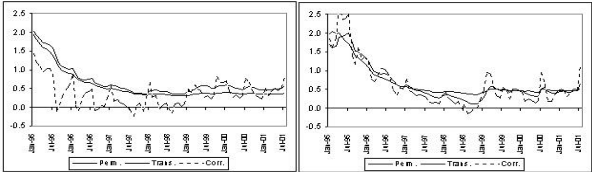
Figure 4: E(\hat{\theta}_t^h) for Normal Models T, P, C and Trim Models
