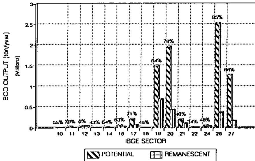
GRAPH 1 INDUSTRIAL BOD OUTPUT BY SECTOR BRAZIL 1988
