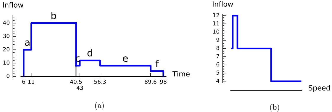
Figure 6: On the left the plot showing the inflow of the network in any given time; the letters indicates the phase to which the outflow is associated to. On the right the plot indicating the relation between the inflow of the network and the speed (inverse travel time) for the agents departing after time 40.5.
