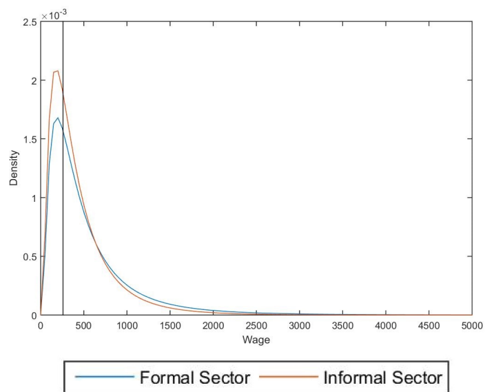
Figure 1: Latent Densities
