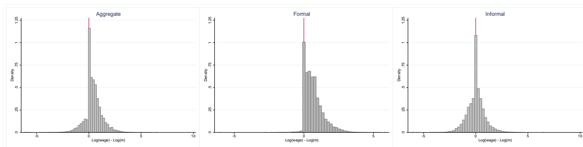
Figure 5: Wage distribution
