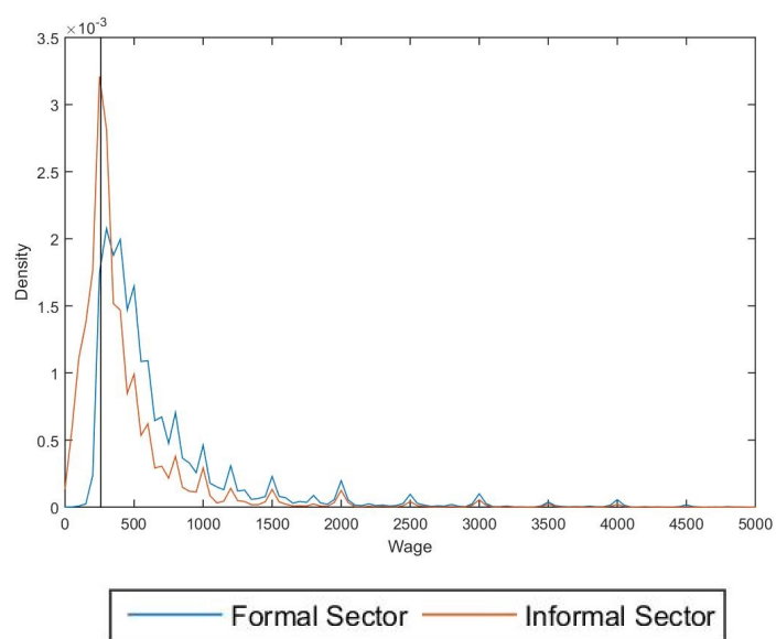
Figure 2: Observed Densities
