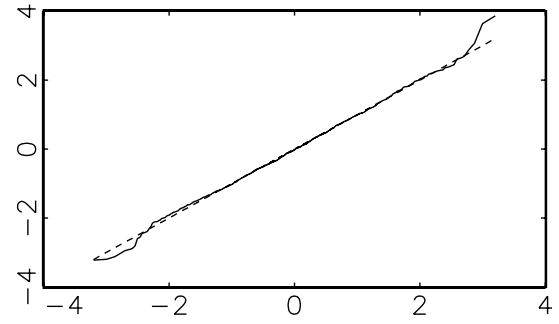
(b) QQ-Plot of z^*
