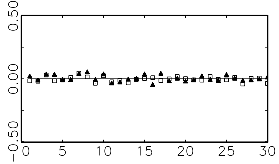
(b) ACF of standardized Pearson residuals z and z^2
