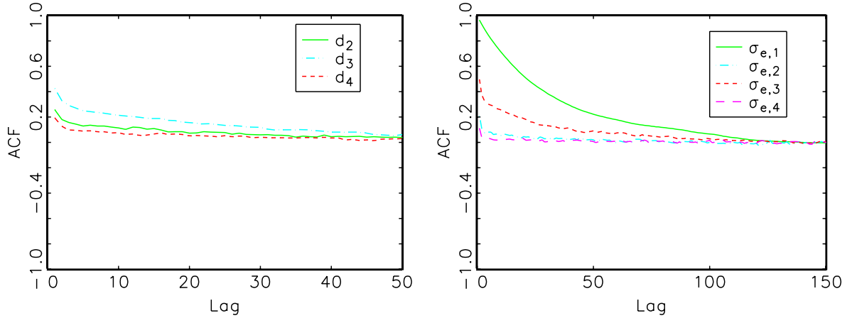
Fig. 3. Autocorrelation functions of the draws of the D and \Sigma_e parameters in the multivariate SV model from 20,000 Gibbs iterations. The functions for d_2 , d_3 , d_4 are in the left panel and for \sigma_{e,1} , \sigma_{e,2} , \sigma_{e,3} , \sigma_{e,4} in the right panel.
