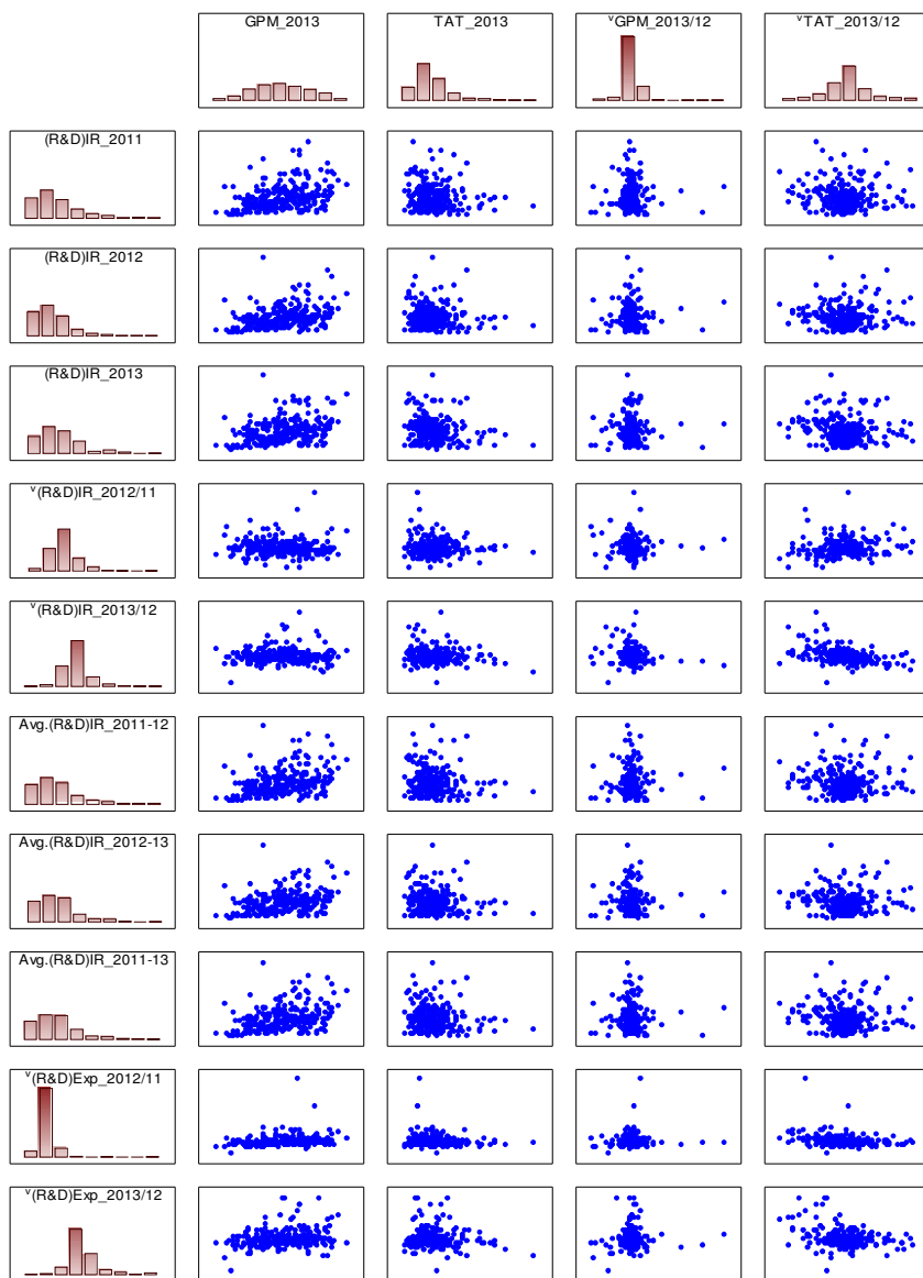
Figure 5. The Scatterplots of assessment criteria pairs from the viewpoint of efficiency measures for the year 2013.
