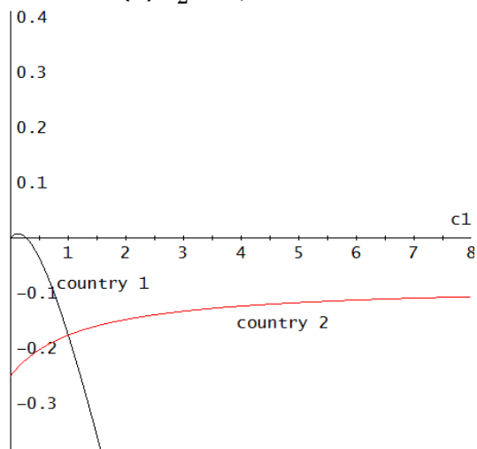
Figure 3. Differential loss L^T_i - L^N_i with increasing policy aversion of country 1
