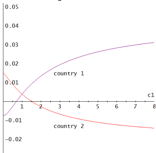
Figure 5. Differential loss L^E_i - L^N_i with increasing policy aversion of country 1
