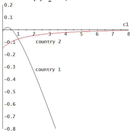
Figure 4. Differential loss L^H_i - L^N_i with increasing policy aversion of country 1
