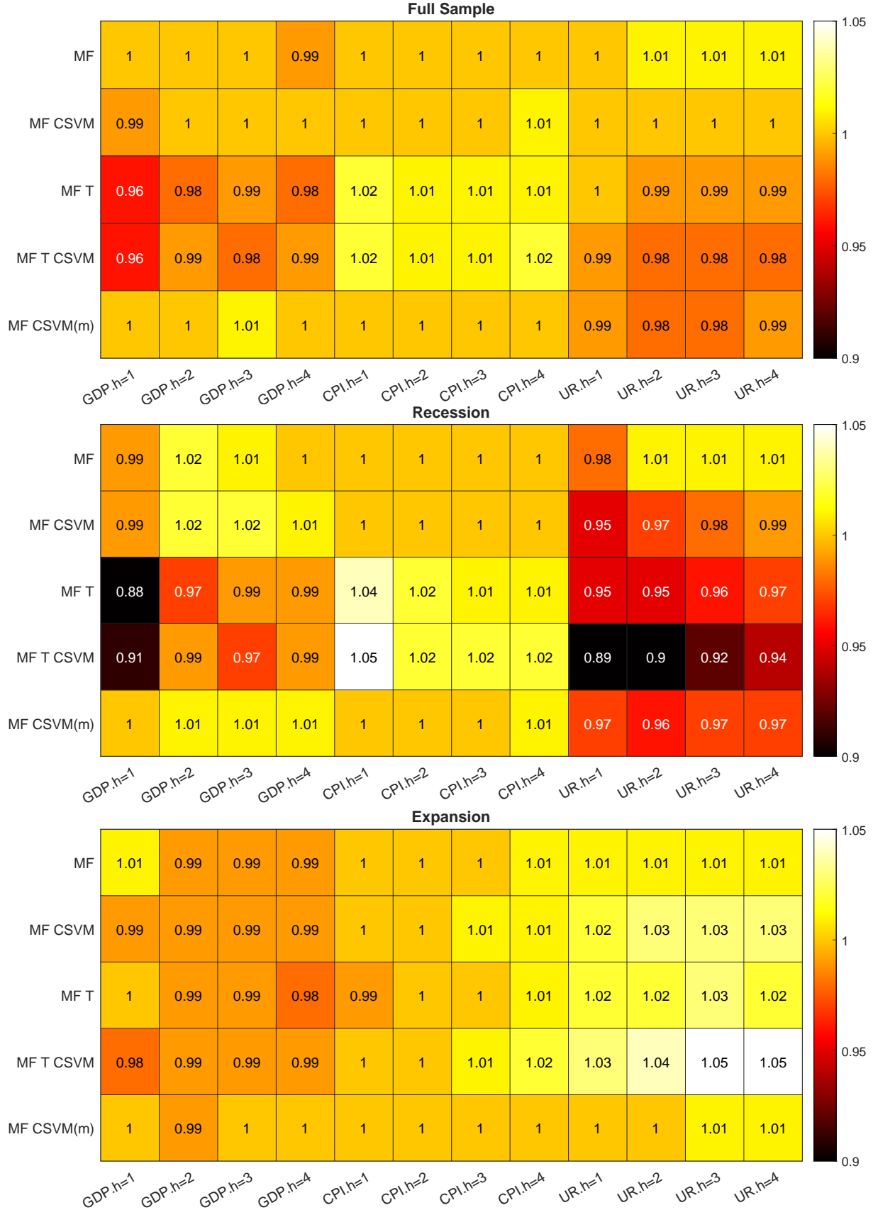
Figure 9: Relative RMSEs - BC Shrinkage against Cross Variable Shrinkage
