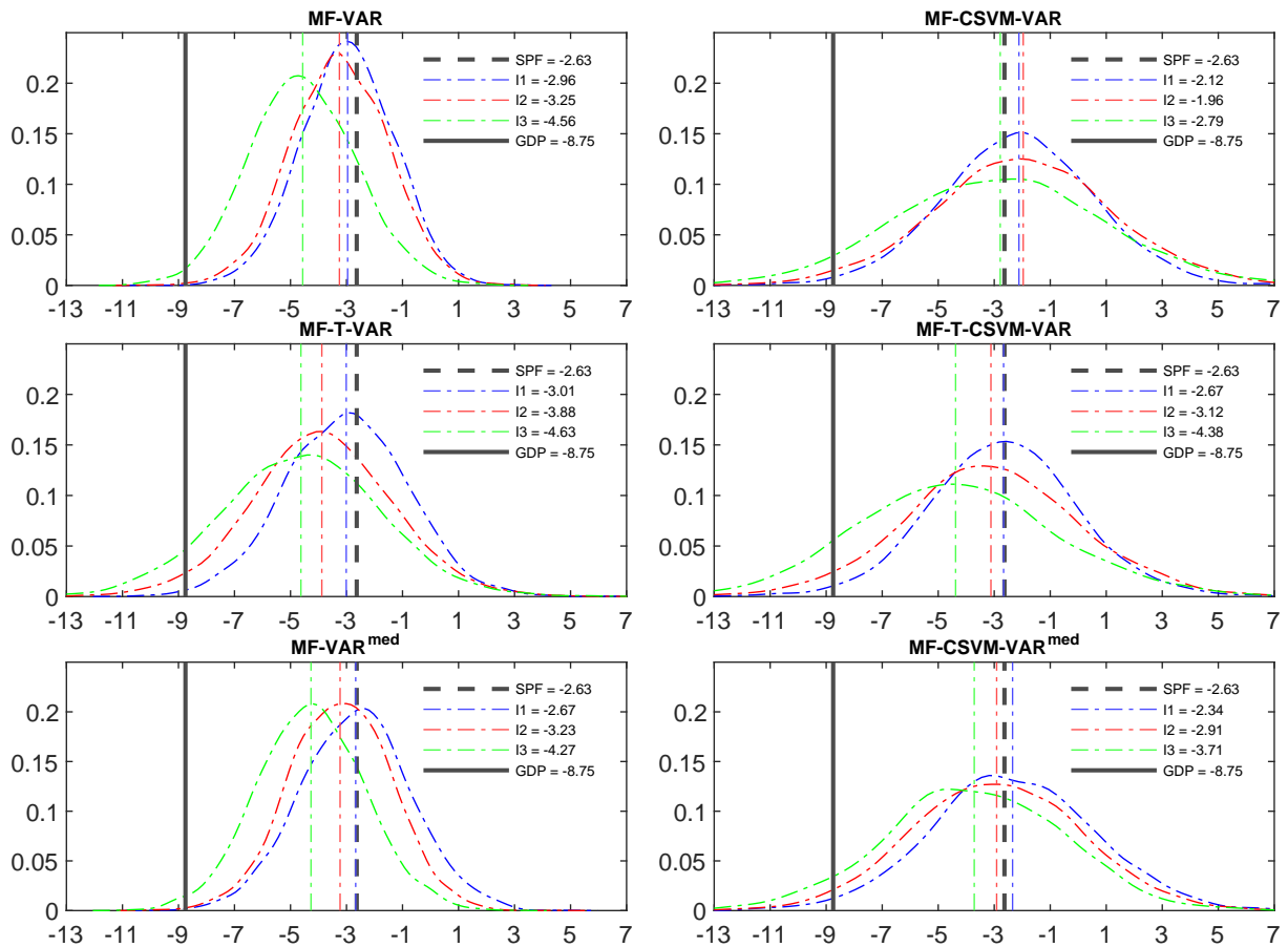
Figure 5: GDP Nowcast Densities for 2008Q4 during the Great Recession
