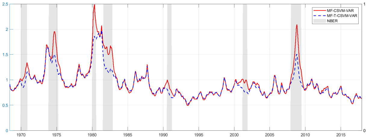
Figure 2: Common Stochastic Volatility
