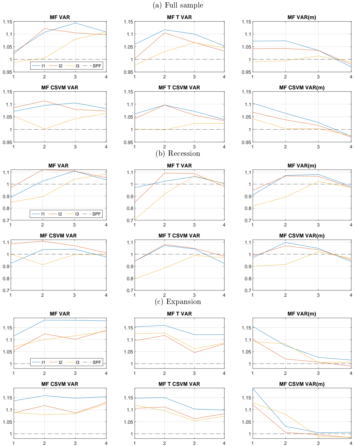
Figure 7: RMSE relative to SPF - GDP
