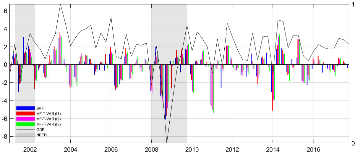
Figure 4: Nowcast Errors - SPF against MF-T-VAR
