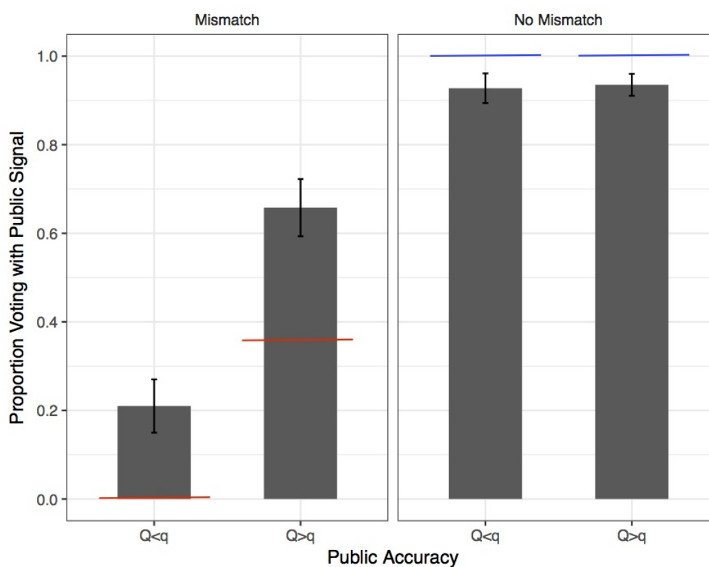
Figure 1. Responsiveness of vote to signals' precision: Average fraction of votes with public signal in sessions with committee decisions, and associated 95% confidence intervals. Standard errors are clustered at the individual level. In the left plot, the public signal and the private signal disagree, and red lines represent the symmetric responsive equilibrium prediction for \mu , the probability of voting for the public signal under mismatch. In the right plot, the signals agree, and blue lines represent the unique optimal decision when the two signals agree.
