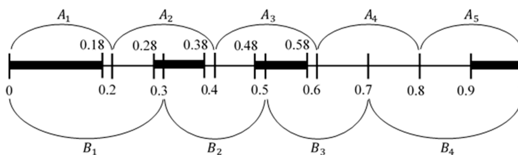
Figure 2. Information sets for more complex example.
