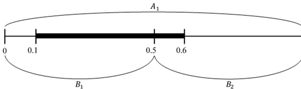
Figure 1. Information sets for simple example.
