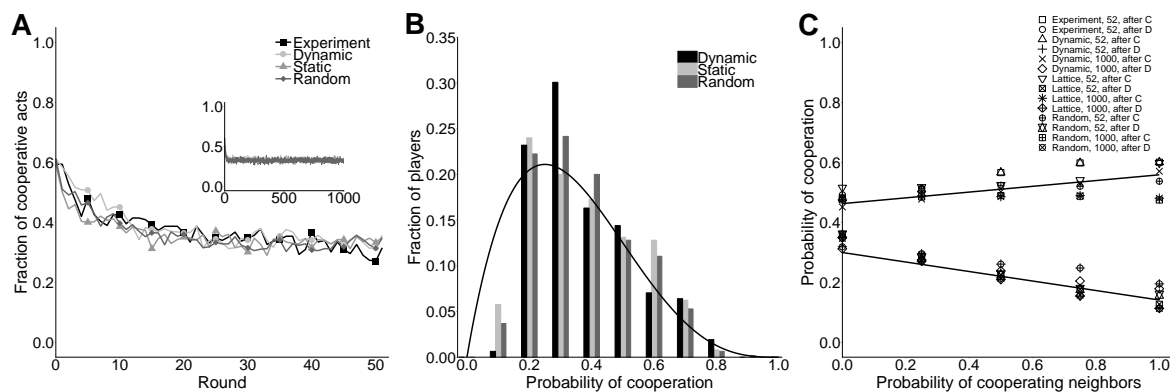
Figure 1. Simulation of Zaragoza’s experiment. (A) Fraction of agents who cooperated in each round of the game on the Zaragoza experiment (black line with square), dynamic lattice treatment (light gray line with circle), static lattice treatment (medium gray line with triangle) and regular random network treatment (dark gray line with diamond). The inset shows the same results for a larger number of rounds. (B) Fraction of agents that reached a certain probability of cooperation in the game on the dynamic lattice treatment (black), static lattice treatment (light gray) and regular random network treatment (dark gray). The continuous black line shows the Ansatz \mu(P) = 2P(1 - P)^3 described in Appendix A. (C) Probability for a generic agent to cooperate after she cooperated (after C) or after she defected (after D) in the three different treatments (Dynamic, Lattice and Random) assuming the length of the simulation is 52 or 1000 rounds. The straight black lines with positive and negative slopes show, respectively, the MCC values for after C and after D obtained by using the Ansatz \mu(P) and the equations described in Appendix A.
