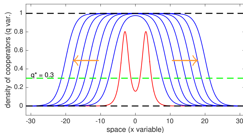
Figure A2. The figure shows another numerical simulation in 1D where the initial datum is a two peaked cluster, namely: q_0 = \frac{0.8}{\cosh(x-3)} + \frac{0.8}{\cosh(x+3)} . Even if in a certain interval of the initial datum's domain cooperators are below the threshold they can still invade the whole space.
