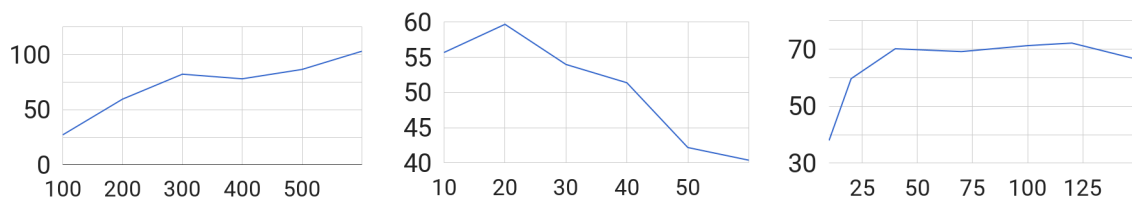
Figure 5. The number of iterations ( y -axis) as |V| , k , and |W| increase ( x -axis).
