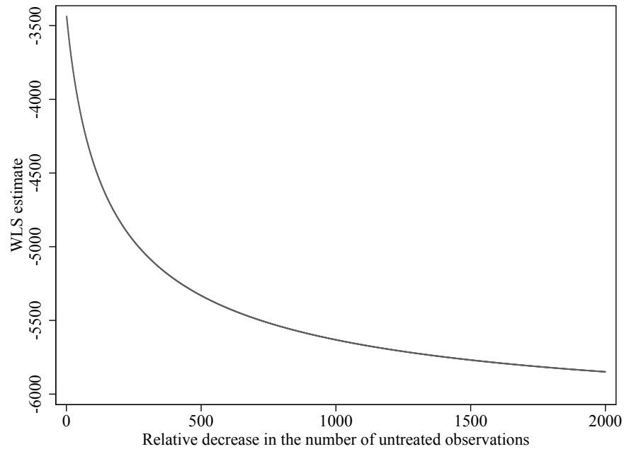
Figure E1.1: WLS Estimates of the Effects of a Training Program on Earnings
