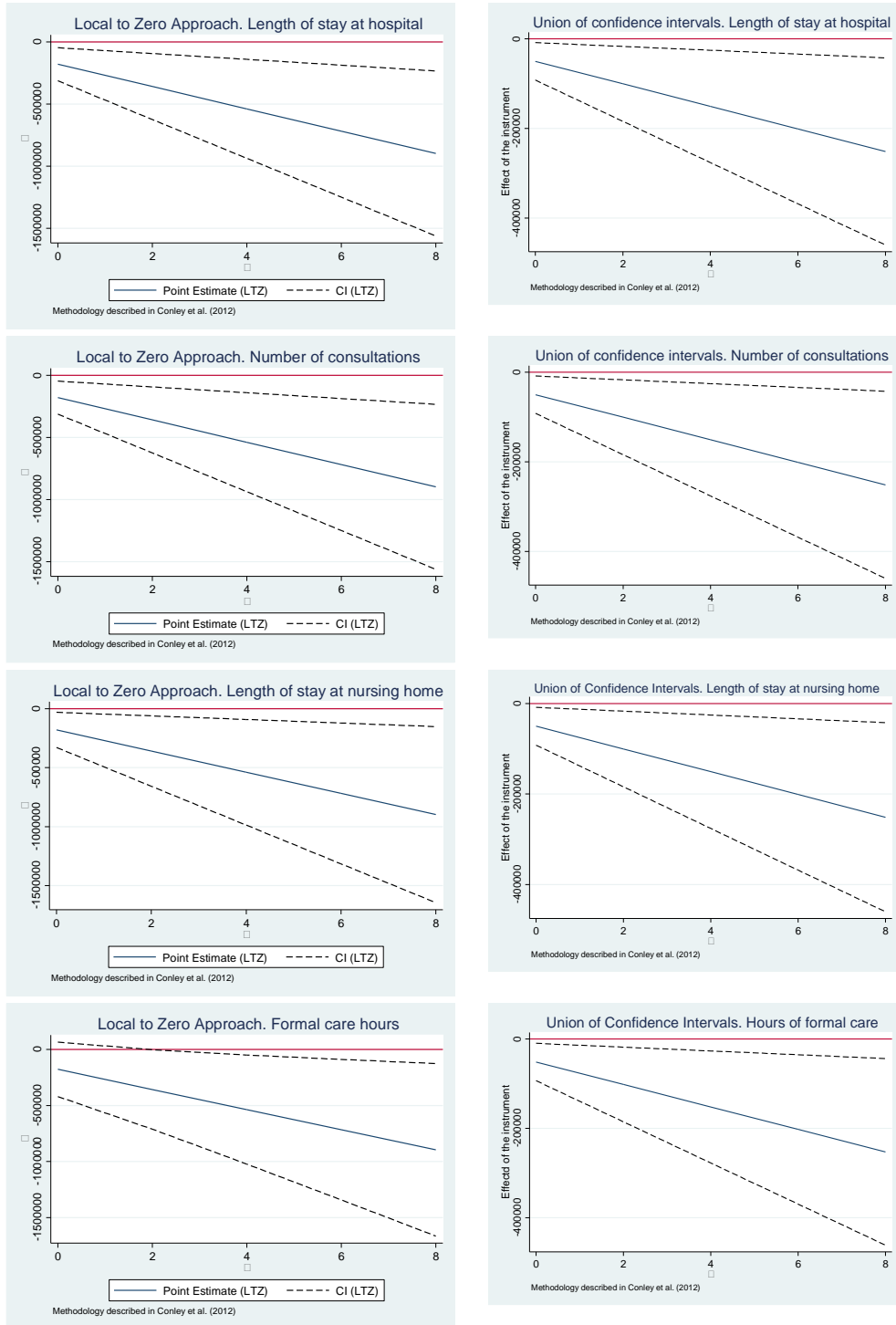
Figure D1. Local-to-Zero approximation and Union of Confidence Intervals. Test for instrument validity.
