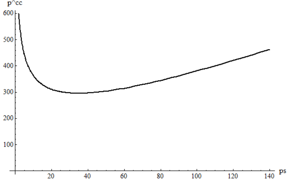
Figure 2: Optimal price level with carbon contracts as a function of p_s for d = 200 , c = 0
