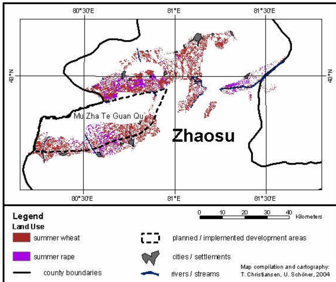
Fig. 33: Classification results for rainfed land ("glebe") in area Southwest
